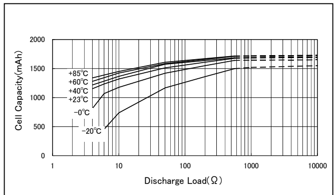
Discharge Load vs. Cell Capacity of CR17335E-N
