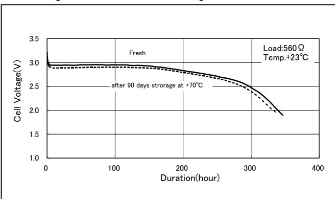
Discharge Characteristics after storage of CR17335E-N
